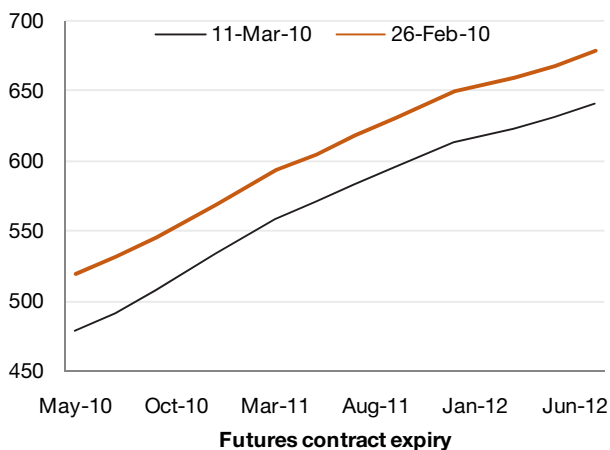
Figure 1: Chicago wheat futures curve (US$/bu)
