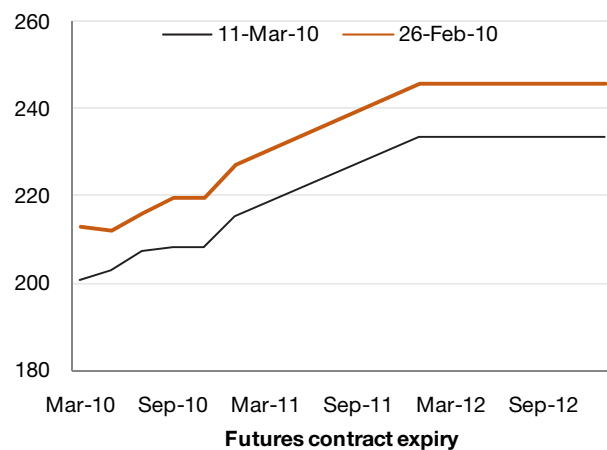
Figure 2: ASX NSW wheat curve (A$/t)
